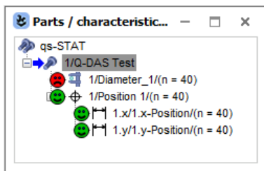
Data set structure before upload
